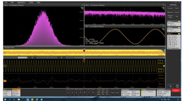
Jitter Measurement using DPOJET
