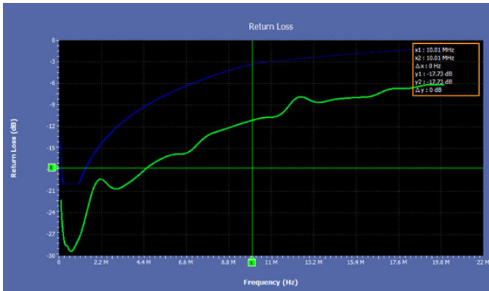
Return loss plot generated using oscilloscope and AWG method
