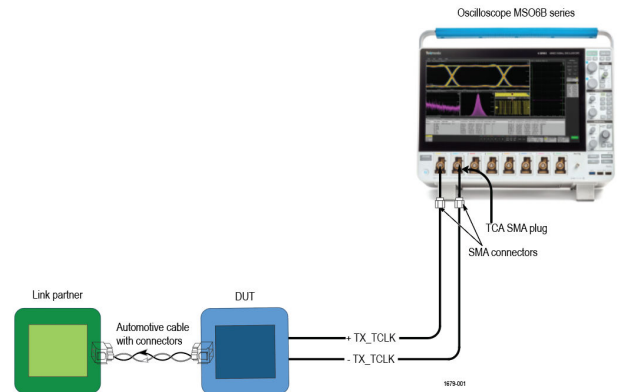
Automotive Ethernet connection diagram
