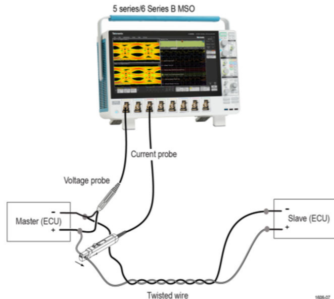
Software based signal separation configuration
