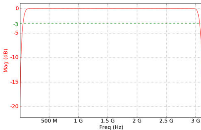
Hilbert response
