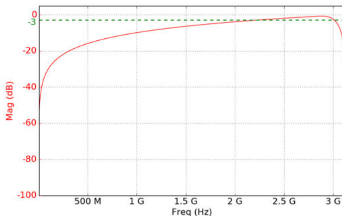
Differentiator response
