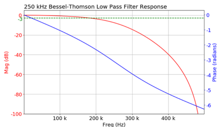
Bessel-Thompson response
