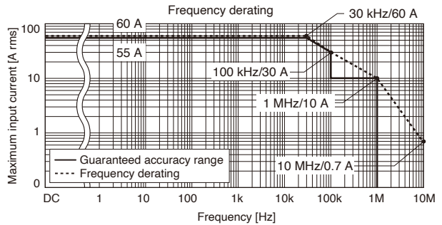
Frequency characteristics (example of typical characteristics)
