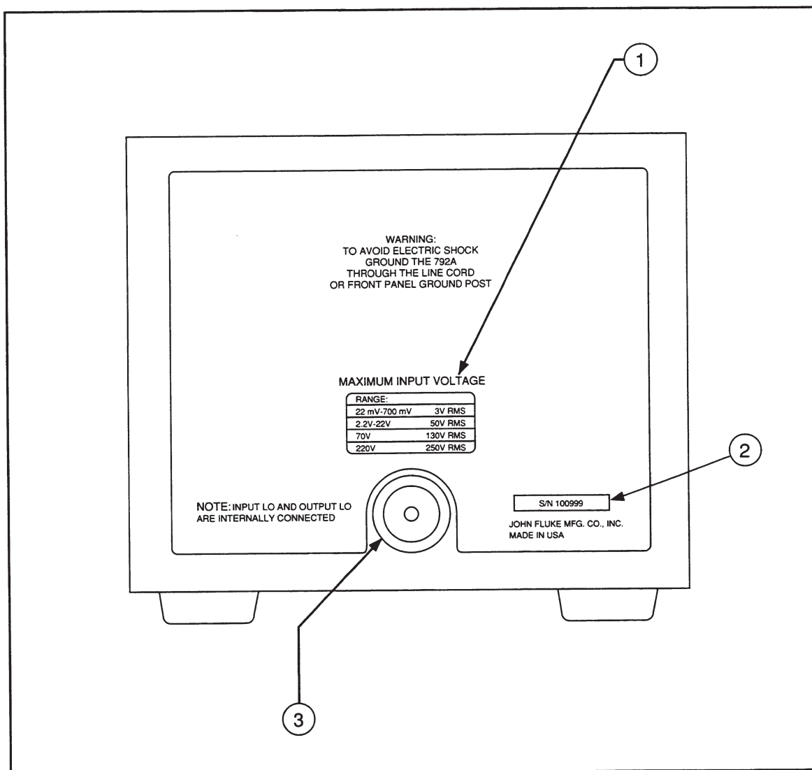
Figure 3-2. 792A AC/DC Transfer Standard Rear Panel
