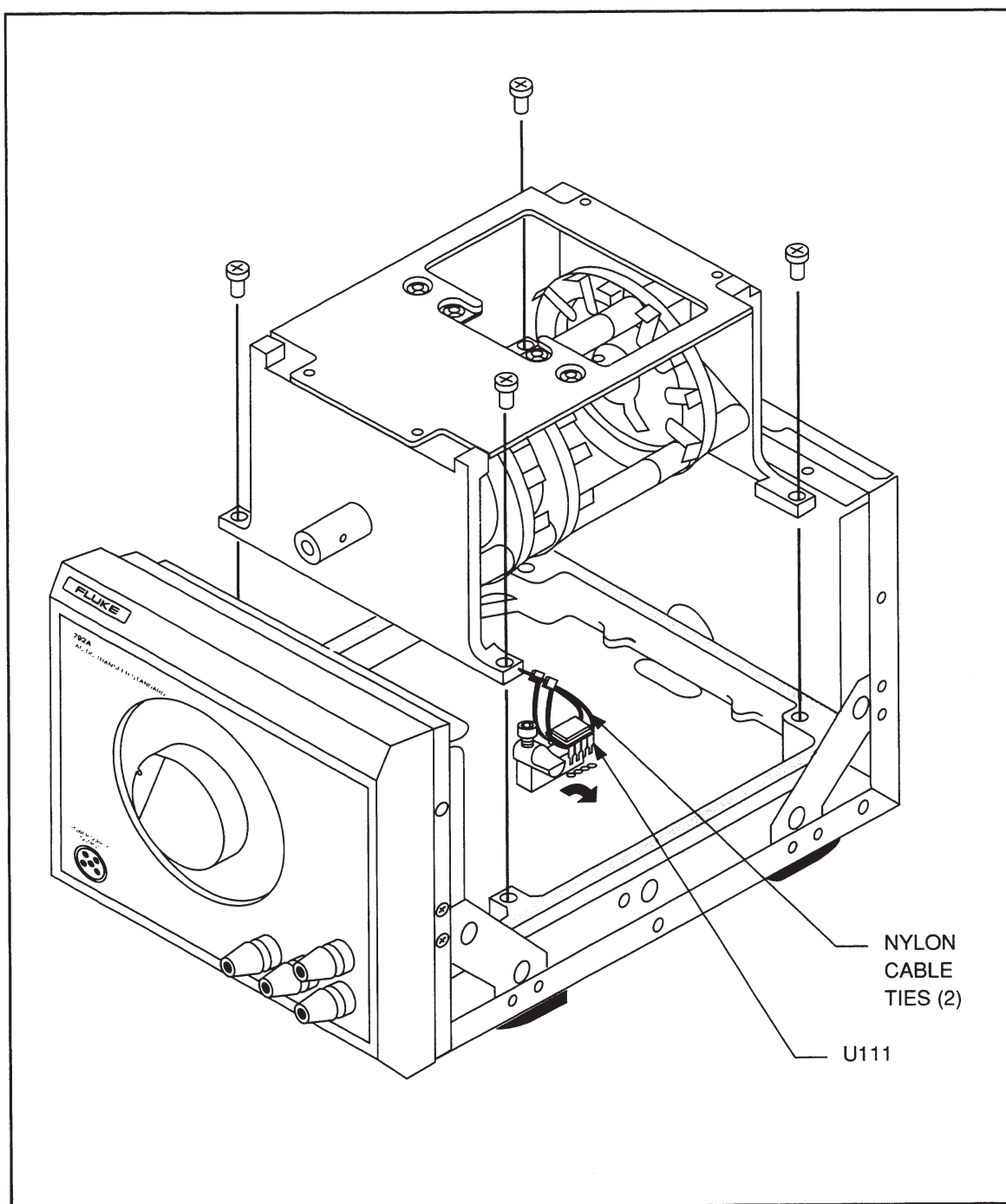
Figure 5-4. Replacing U111
