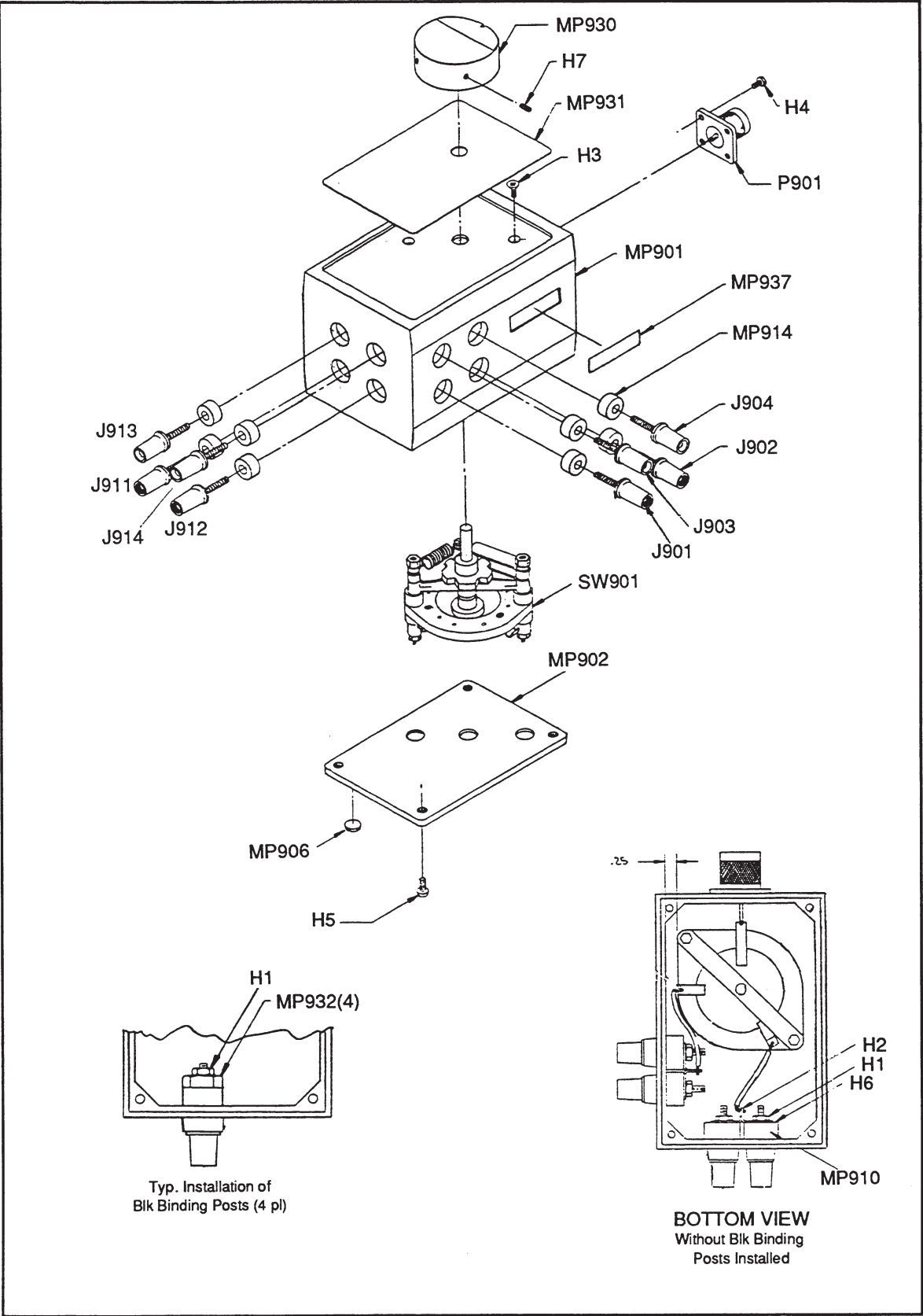
Figure 6-7. Transfer Switch
