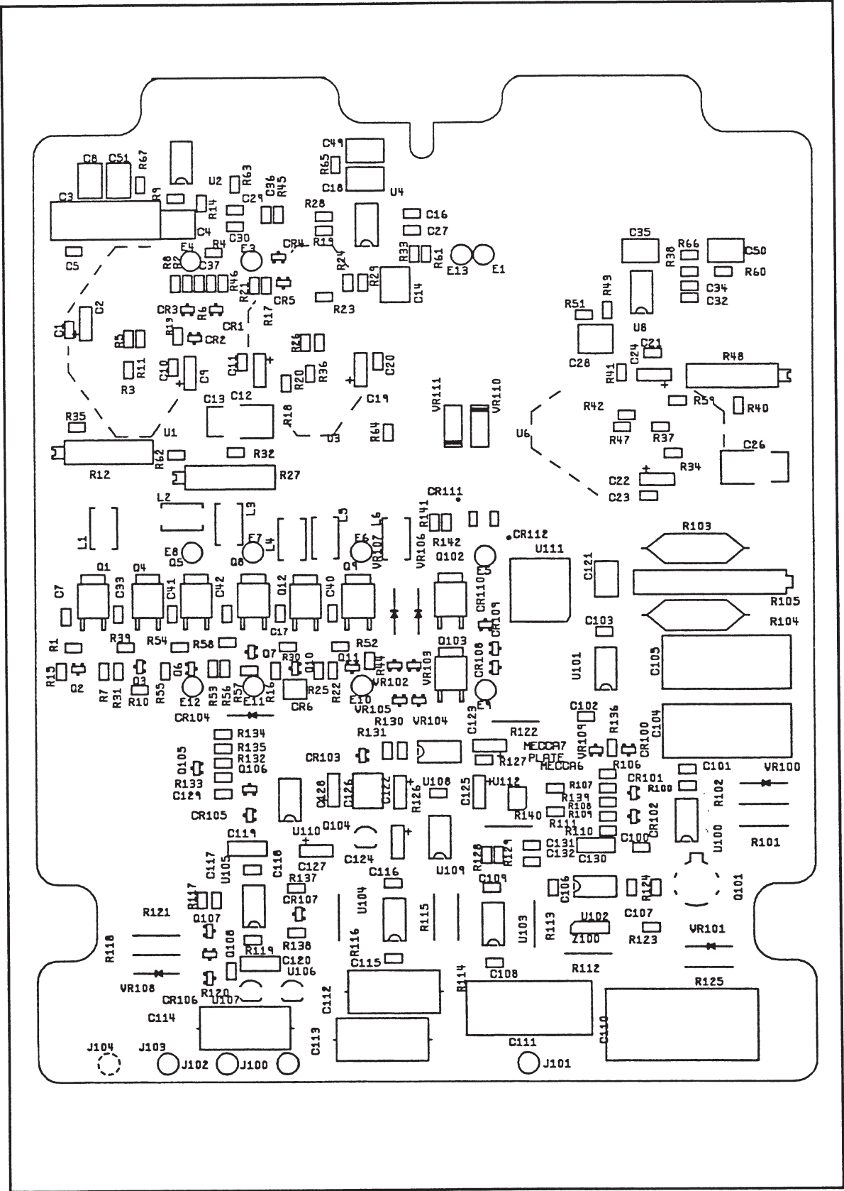
Figure 6-3. A2 Sensor PCA
