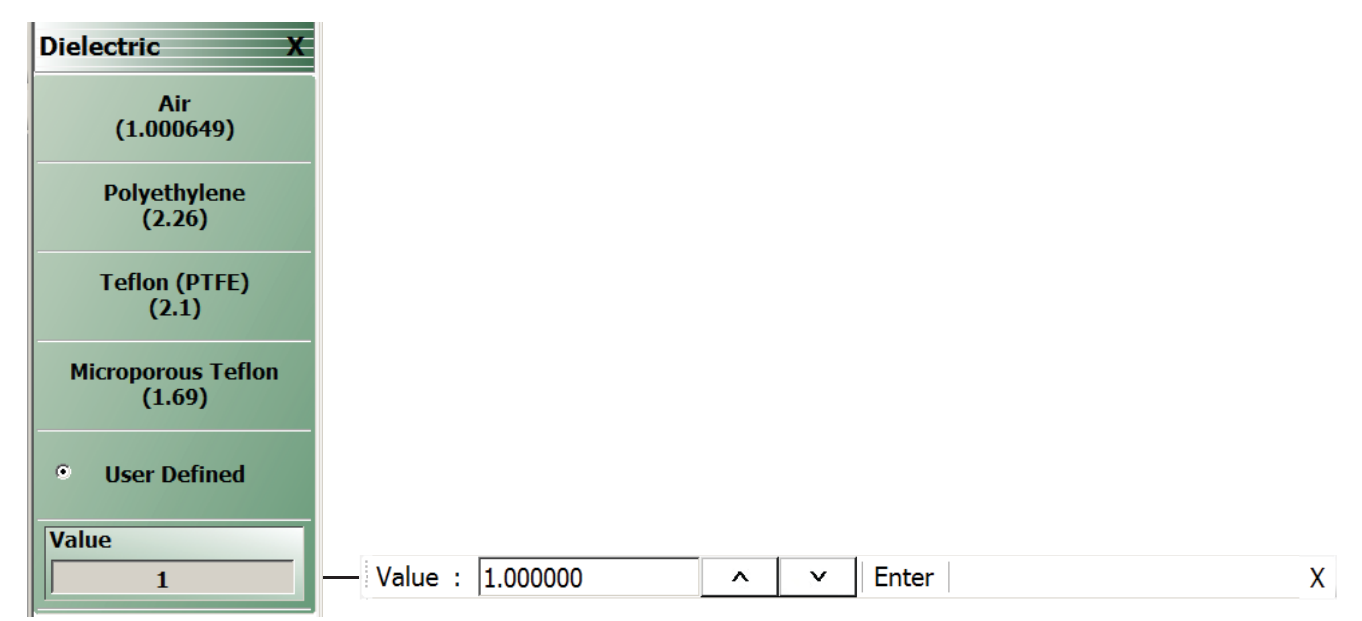
Figure 9-24. DIELECTRIC Menu
