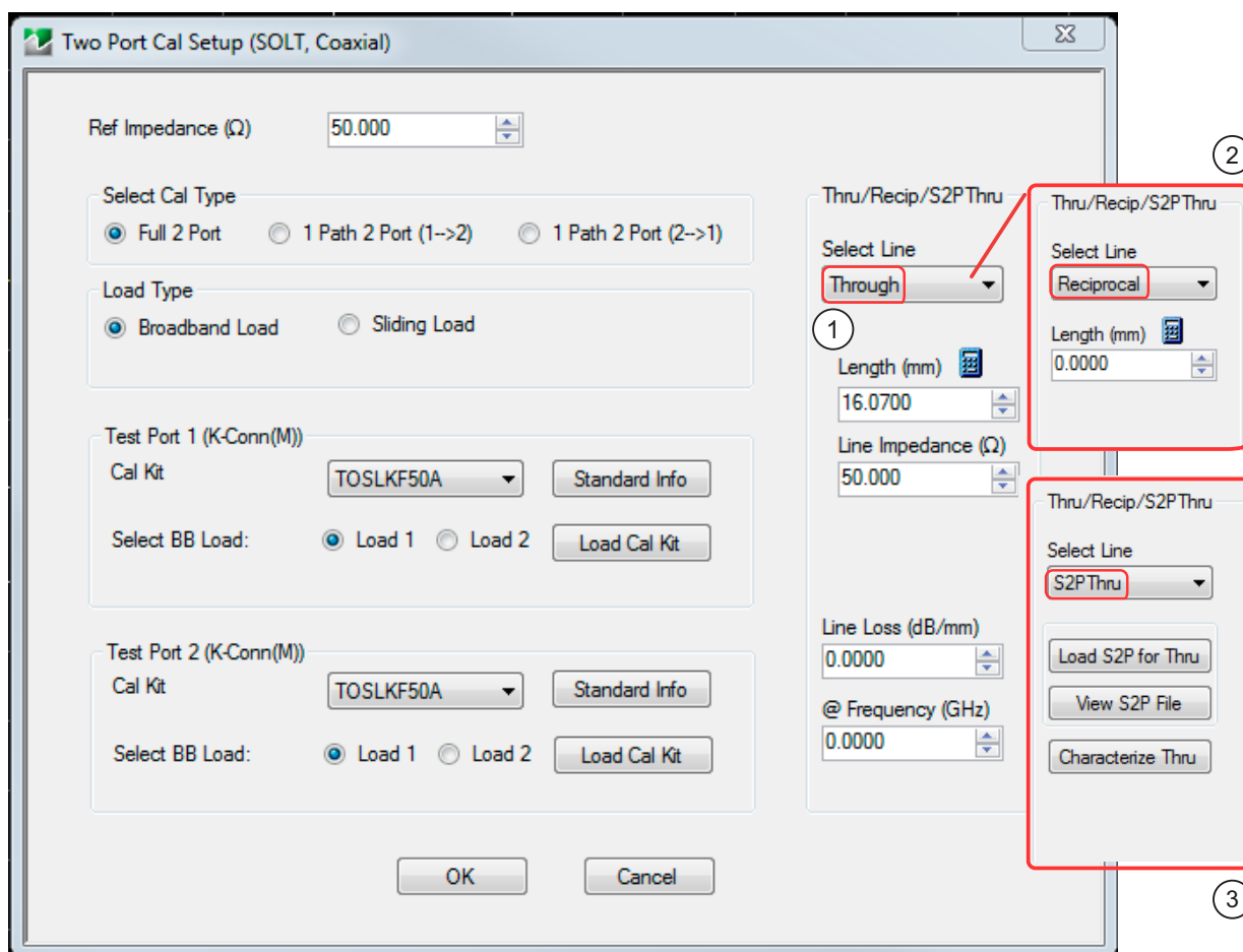
Figure 8-55. Edit Cal Params – TWO PORT CAL SETUP (SOLT, COAXIAL) Dialog Box
