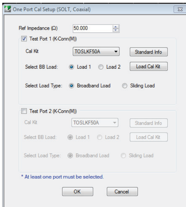
Figure 8-64. ONE-PORT CAL SETUP (SOLT/SOLR, COAXIAL) Dialog Box
