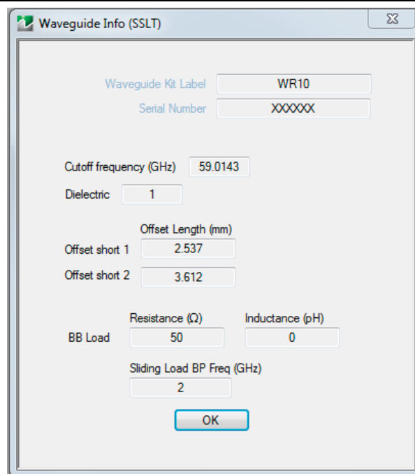
Figure 8-84. USER DEFINED WAVEGUIDE Dialog Box
