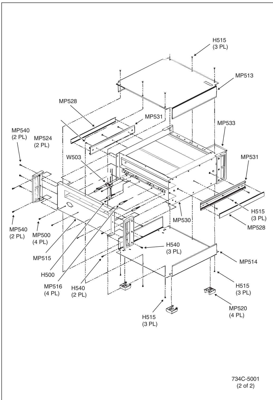
Figure 19. 734C DC Reference Standard (cont)
