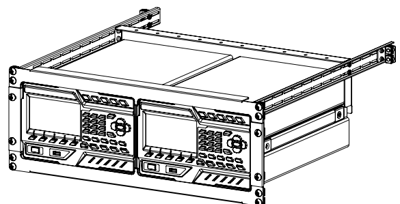
Rack Mount Kit (Two Instruments)
