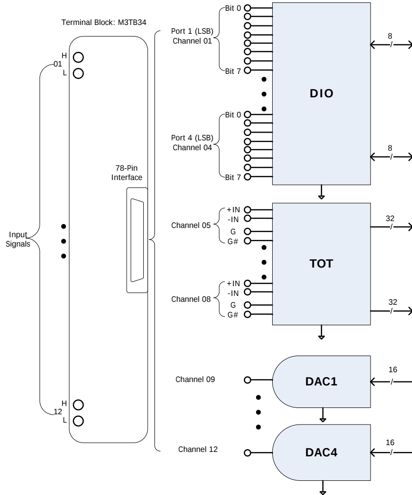
Figure 28 MC3534 Schematic Diagram
