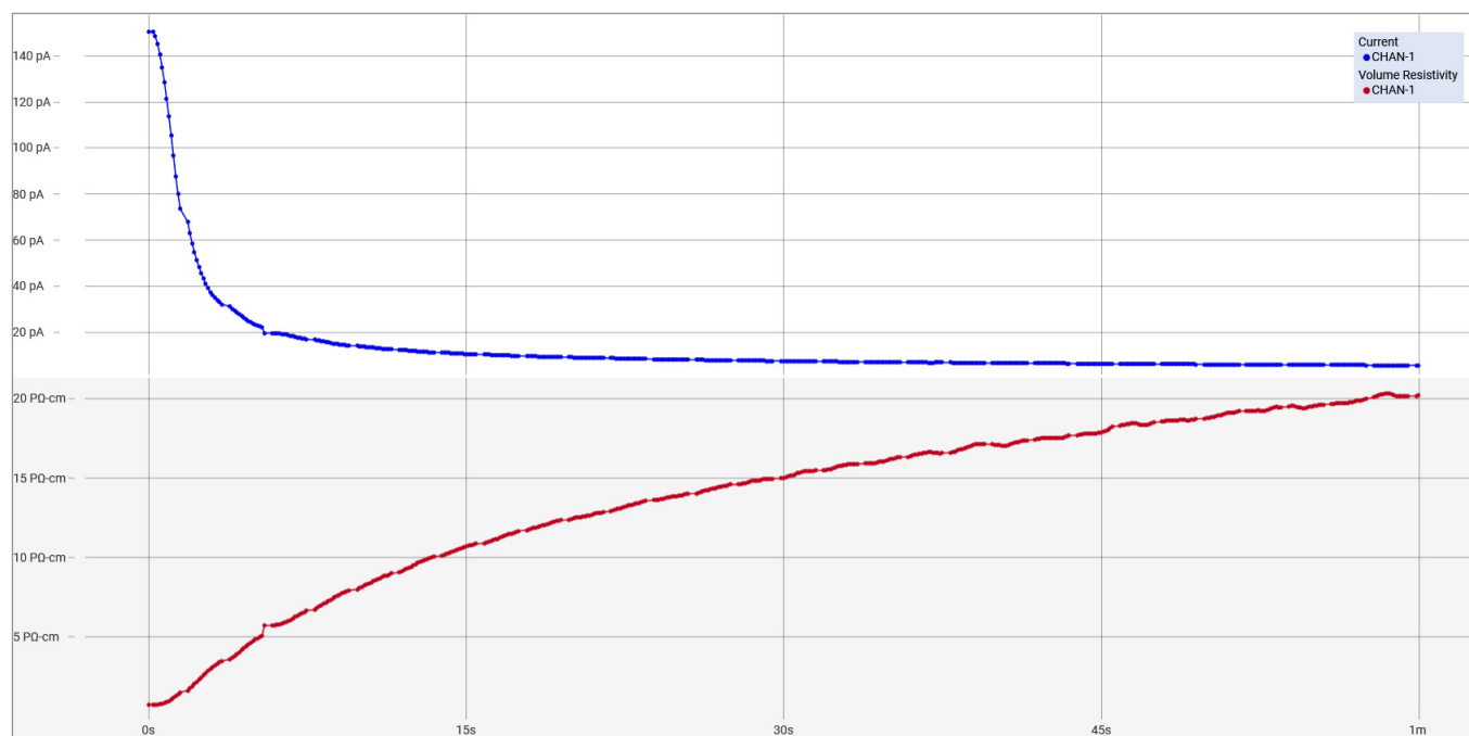
KickStart High Resistivity resistivity plot
