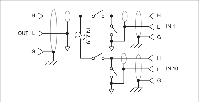
6522 schematic.
