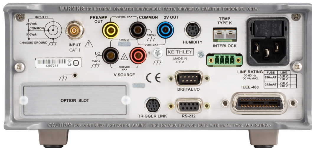
6517B rear panel.
