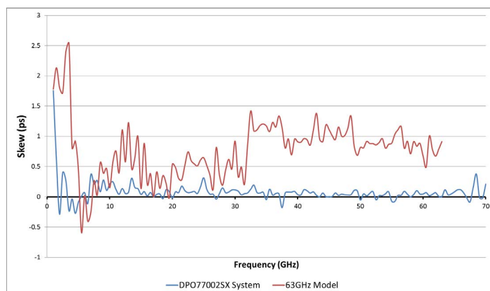
Channel skew vs. Frequency comparison between DPO7002SX system and other vendor's 63 GHz model.
