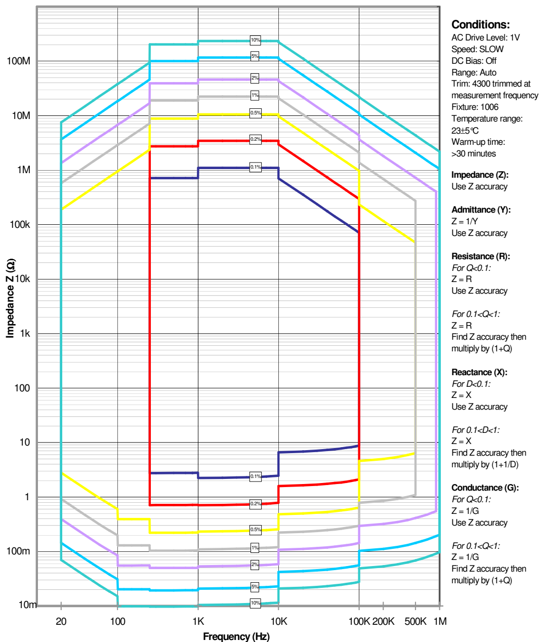
4300 Impedance Measurement Accuracy
