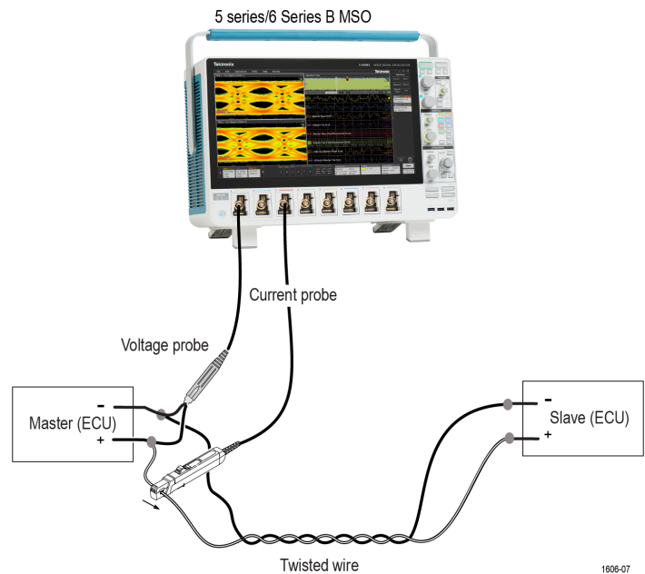
Figure 1: 100BASE-T1 Signal Separation setup
