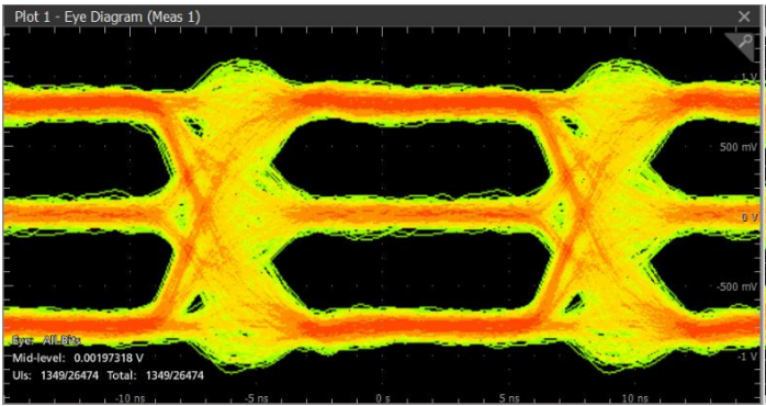
Figure 7: Eye diagram after performing CTLE
