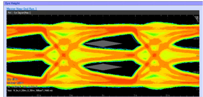
Figure 12: Eye Mask test
