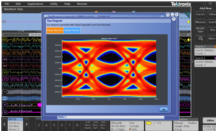
Figure 22: 100BASE-T1 Eye diagram on PC based TekScope Application
