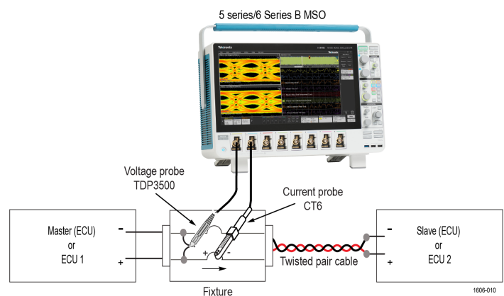
Figure 2: Automotive Ethernet Signal Separation using Fixture
