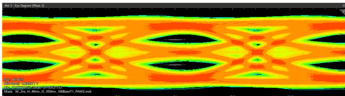
Figure 10: Automotive Ethernet 100BASE-T1 Receiver Eye diagram
