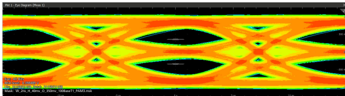
Figure 9: Automotive Ethernet 100BASE-T1 Transmitter Eye diagram
