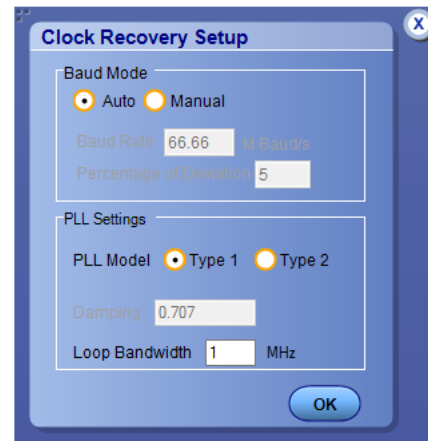
Figure 5: Clock recovery
