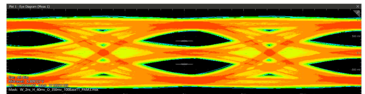
Figure 17: Eye diagram of a three meter cable
