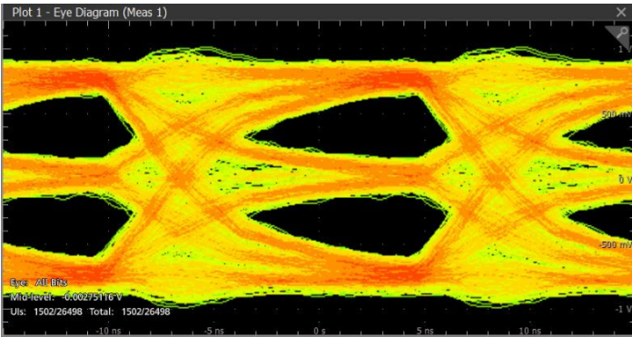
Figure 6: Eye diagram before performing CTLE
