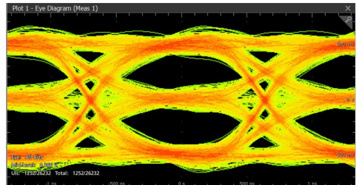
Figure 13: Automotive Ethernet 1000BASE-T1 Transmitter Eye
