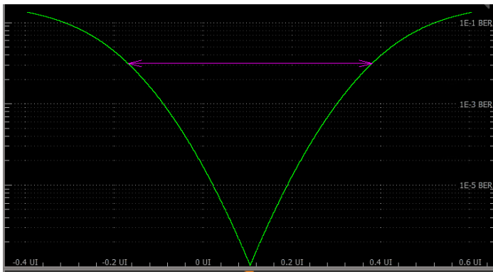
Figure 11: BER Bathtub plot
