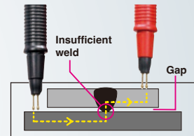
Defective weld
