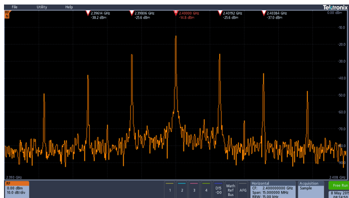
Automated peak markers identify critical information at a glance. As shown here, the five highest amplitude peaks that meet the threshold and excursion criteria are automatically marked along with each peak's frequency and amplitude.
