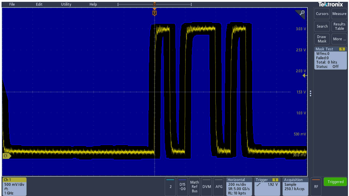
Mask/Limit test example
