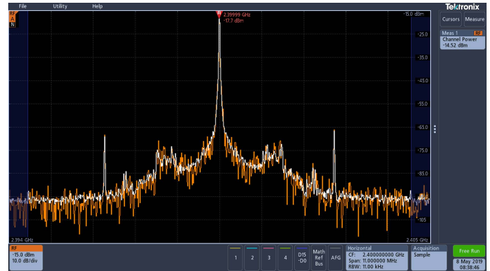
Automated Channel Power measurement
