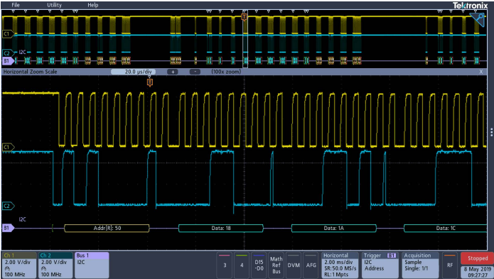
Triggering on a specific address and data packet going across an I 2 C bus. The yellow waveform is clock and the blue waveform is the data. A bus waveform provides decoded packet content including Start, Address, Read/Write, Data, and Stop.
