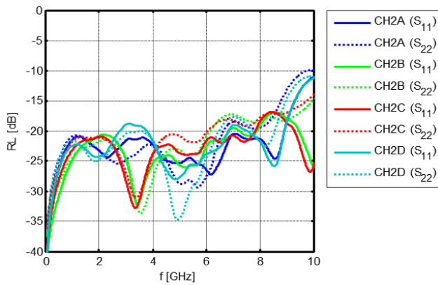
Fig. 5: Return loss (RL) of CH2-input (S 11 ) when routed to 50Ω-terminated output CH2<X> port (S 22 ).
