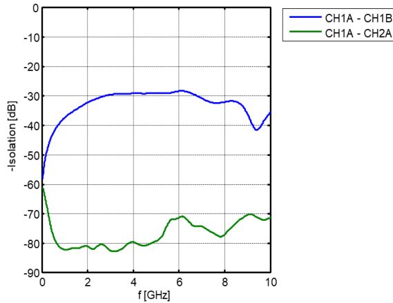
Fig. 7: Isolation between CH1B and CH1 (in), with the latter being routed to 50 \Omega -terminated CH1A port (blue). Isolation between CH2A and CH1 (in), with the latter being routed to 50 \Omega -terminated CH1A (green).
