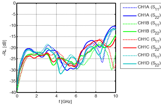
Fig. 3: Return loss (RL) of CH1-input (S 11 ) when routed to 50Ω-terminated output CH1<X> port (S 22 ).
