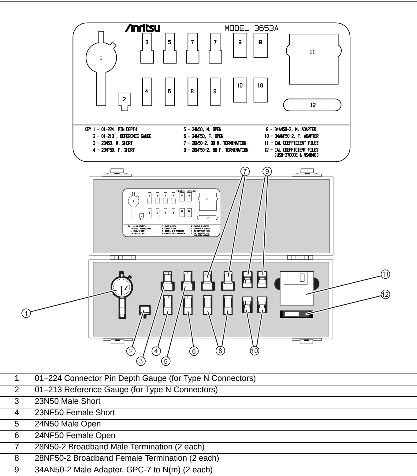
Figure 1-4. Model 3653A N Connector SOLT Calibration Kit (1 of 2)
