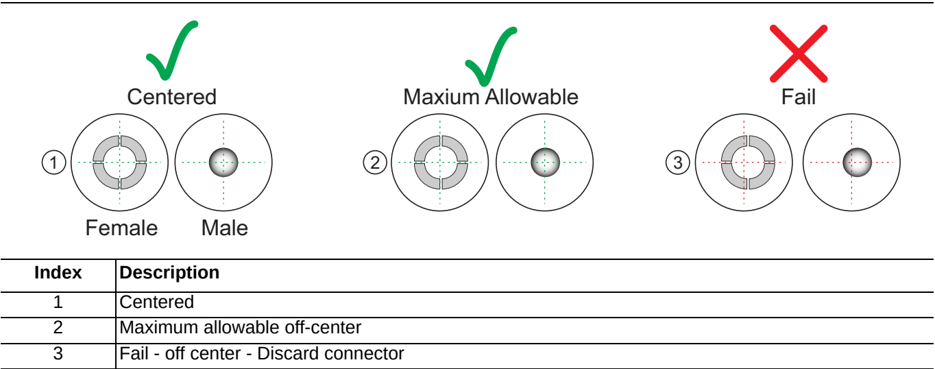
Figure 3-3. Example Connector Concentricity
