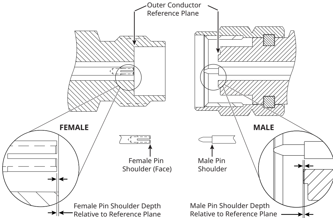
Figure 2-1. 3.5 mm, K, and V Connector Pin Depth Definition
