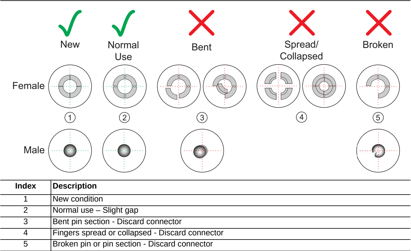
Figure 3-2. Example Connector Damage States
