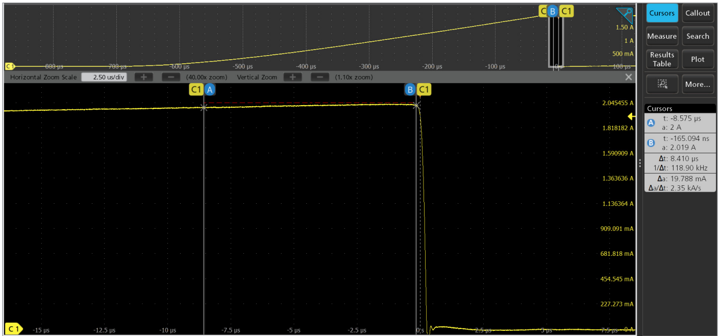
Figure 10: MPSU50-2ST OCP Response Time <50usec
