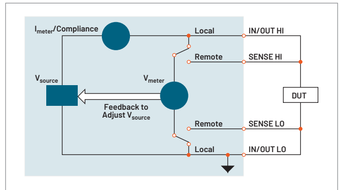
Source V-Measure I, V, or \Omega configuration
