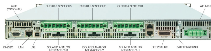
Figure 5. The ASA (pictured) and ASM Series rear panel provides access to analog and digital interfaces.
