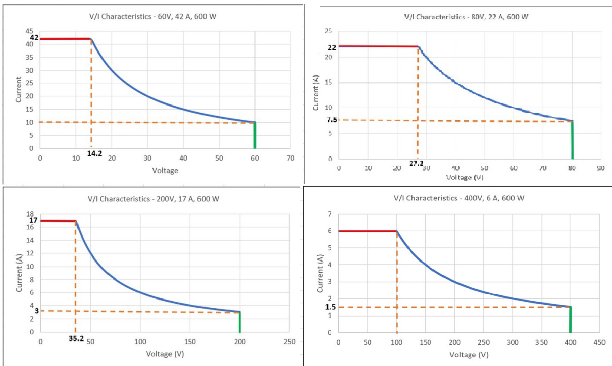
Figure 1. The ASA Series includes four models that follow a 600W I-V curve per channel.
