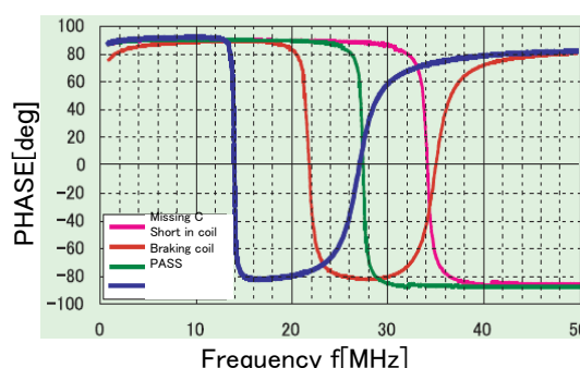
Frequency characteristics of phase
