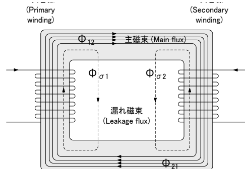
Leakage flux
