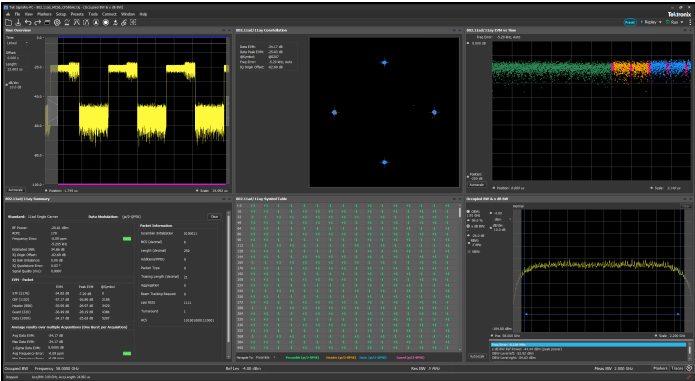
WiGig IEEE802.11ad/ay transmitter testing (offline analysis)
