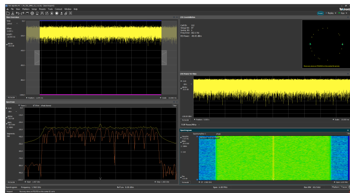
Fast validation of LTE base station transmitter with push button preset, and pass/fail information.
