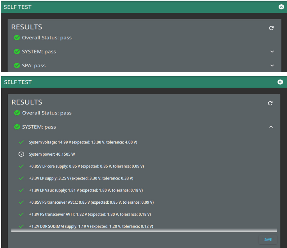
Figure 2-54. Self Test - SPA
