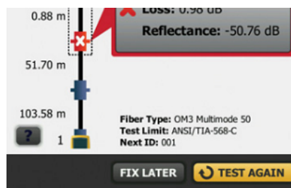
Eventmap – FAIL. See Help icon for on screen corrective action.
