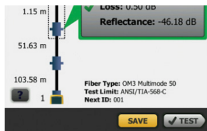
Graphical EventMap view – PASS
