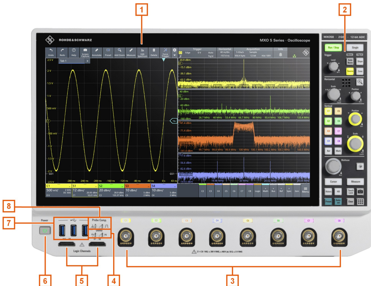
Figure 5-1: Front view of MXO 5 with 8 input channels
