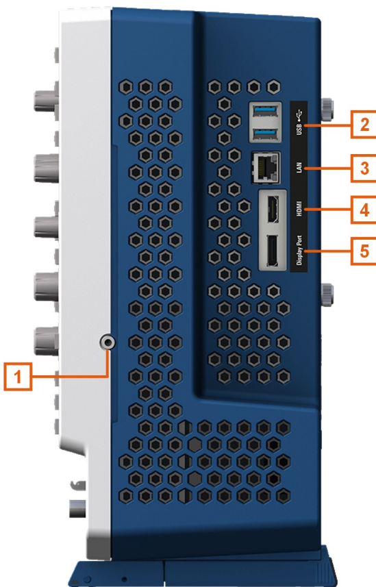
Figure 5-2: Side view of MXO 5
