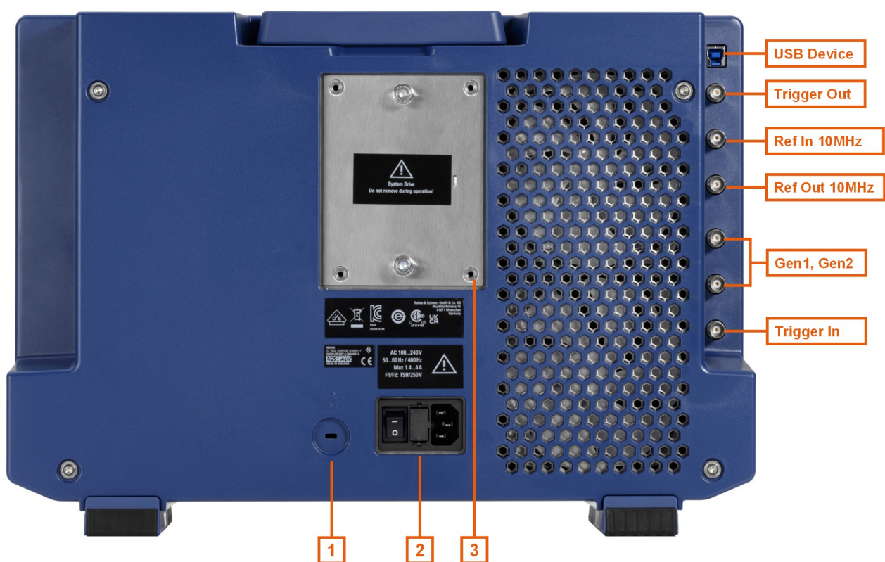
Figure 5-3: Rear panel view of MXO 5
