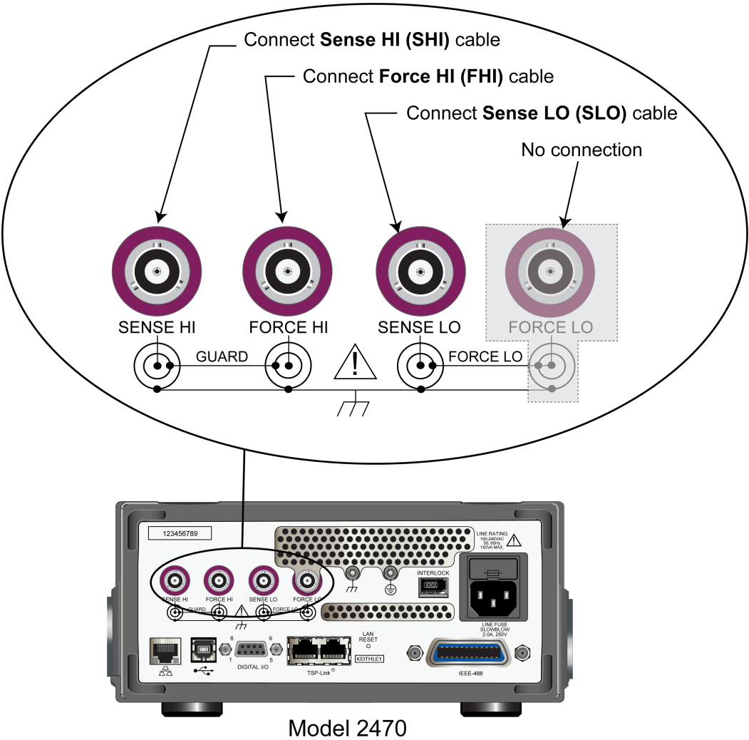
Figure 3: TRX-1100V-BAN cable connection
