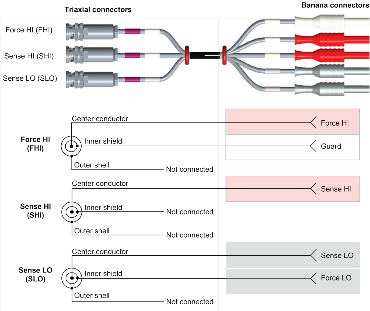
Figure 2: TRX-1100V-BAN cable schematic
