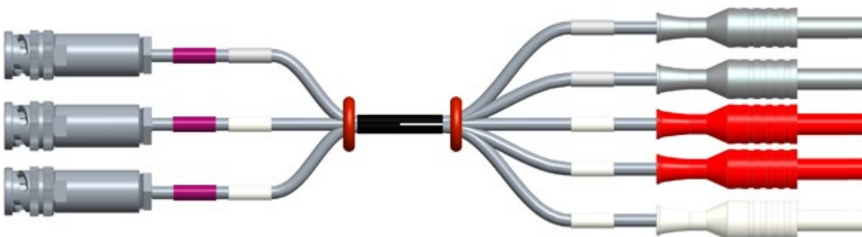
Figure 1: TRX-1100V-BAN cable assembly
