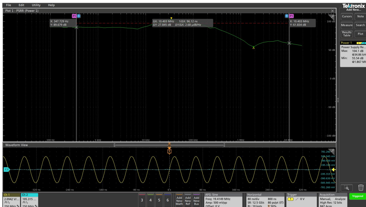
FIGURE 21. The PSRR plot shows the attenuation of AC applied to the input of the supply on the output of the supply.
