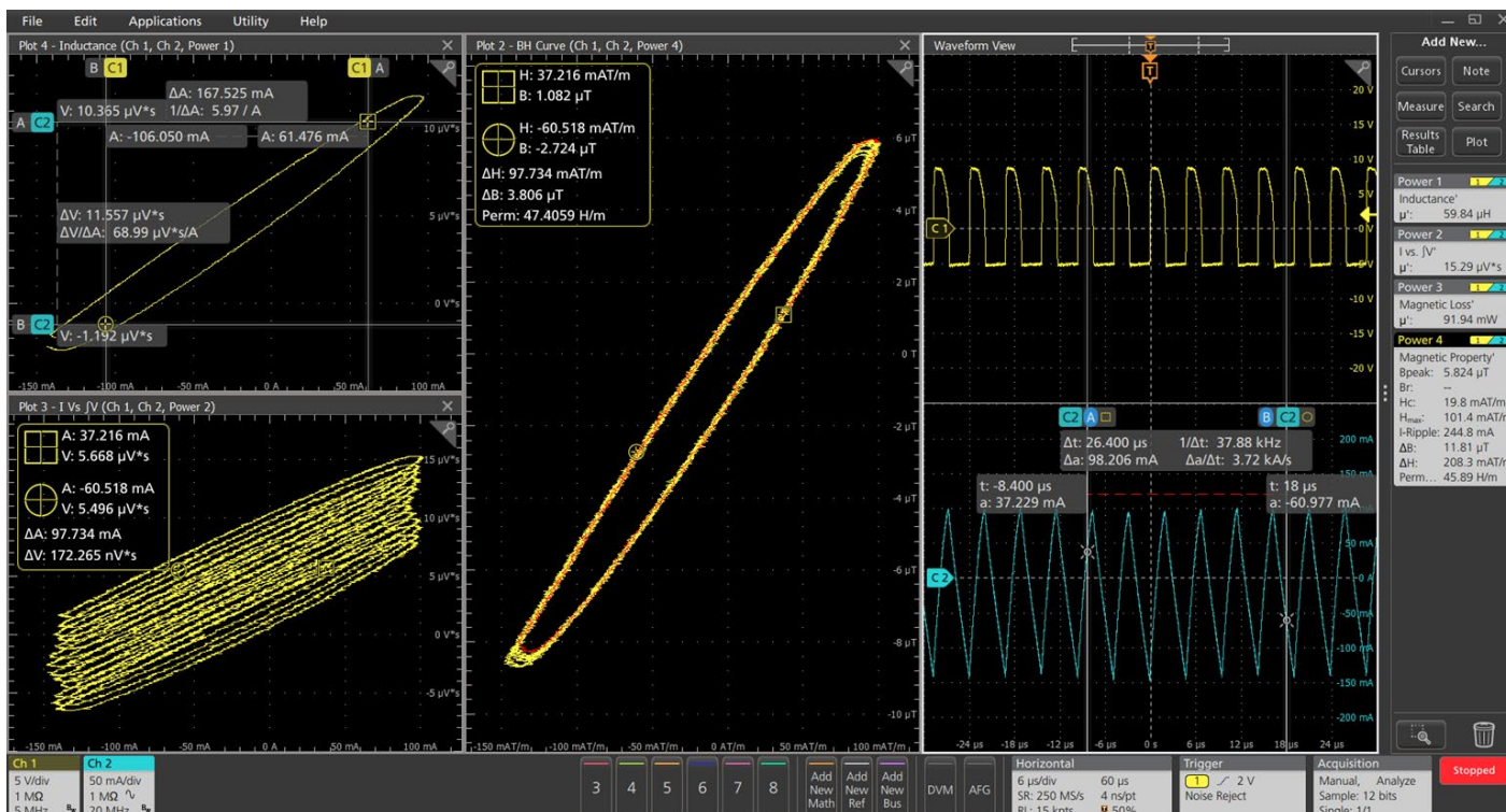
FIGURE 16. Magnetic measurements on an inductor. The Ch1 (yellow) waveform is the voltage across the inductor and the Ch2 (cyan) waveform is the inductor current. The B-H curve is shown in the center of the display. Inductance, magnetic loss, and magnetic properties are shown in results badges on the right.
