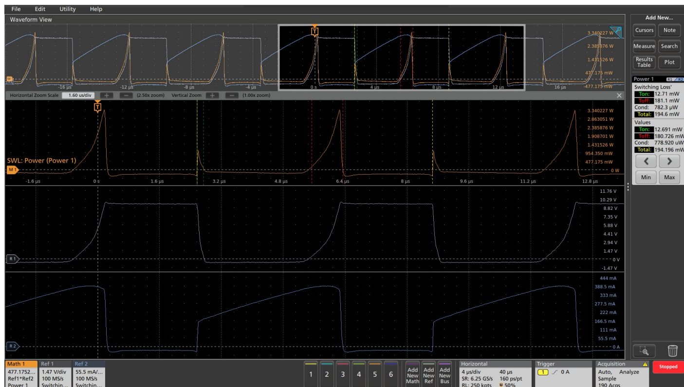
FIGURE 11. Switching Loss Measurements. The upper trace (orange) is calculated by multiplying current and voltage for instantaneous power. Loss measurements are performed on the instantaneous power waveform. Each loss region is annotated with colored markers that correspond to measurement labels. The bottom waveforms are the voltage across the switch and current through the switch.
