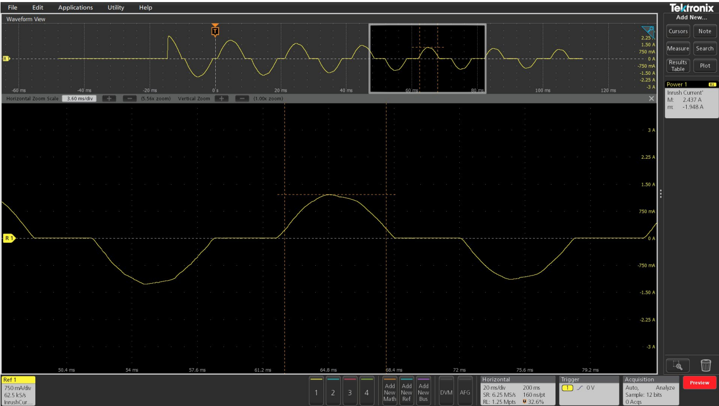
FIGURE 10. Inrush occurs during a power supply turn-on. The current waveform shows gradually reducing peaks before it reaches steady state.
