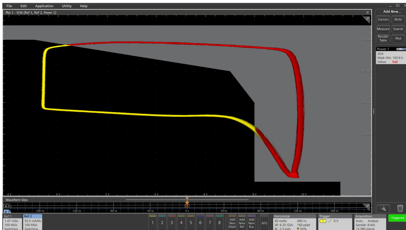
FIGURE 14. SOA using 5-PWR. If the data points fall inside the mask zone, they are yellow to indicate ‘pass’ and if they fall outside the mask zone, they are red to indicate ‘fail’. In this example, the V-I curve has gone outside the SOA, subjecting the switching device to excessive stress.
