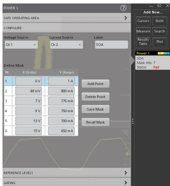
FIGURE 15. SOA Mask Editor window. The mask is defined by a set of (voltage, current) coordinates taken from the switching device datasheet, or may be user-defined.
