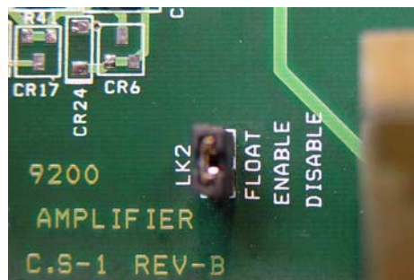
Figure 2-2. Float Enable/Disable Jumper LK2
