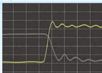
Waveform of an inverter when switched ON
