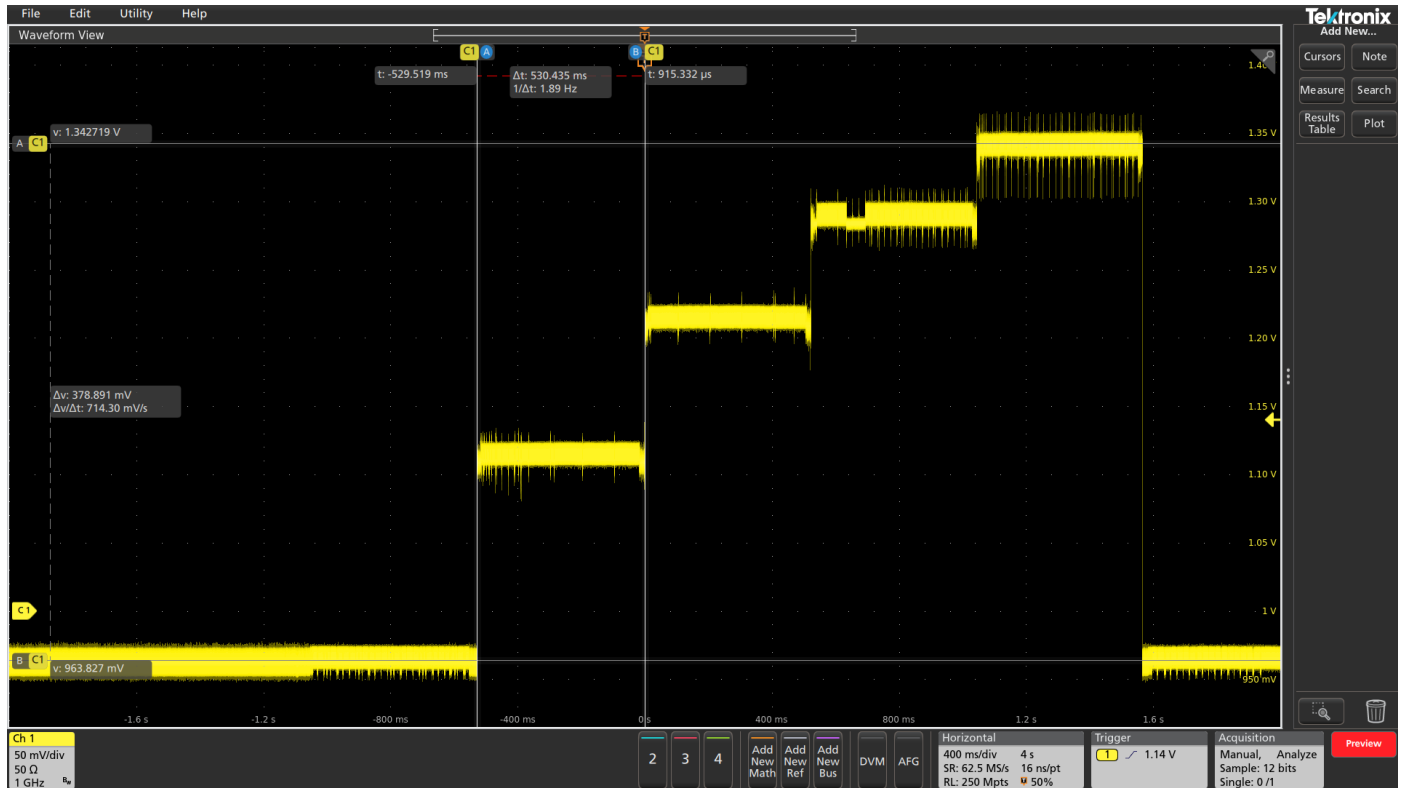
Figure 11. Example of a device that is scaling the input voltage needed as the frequency is increased. The \sim 2 Hz frequency component between steps will be missed with many AC coupling filters
