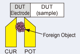
Probe Short-Circuit Detection
