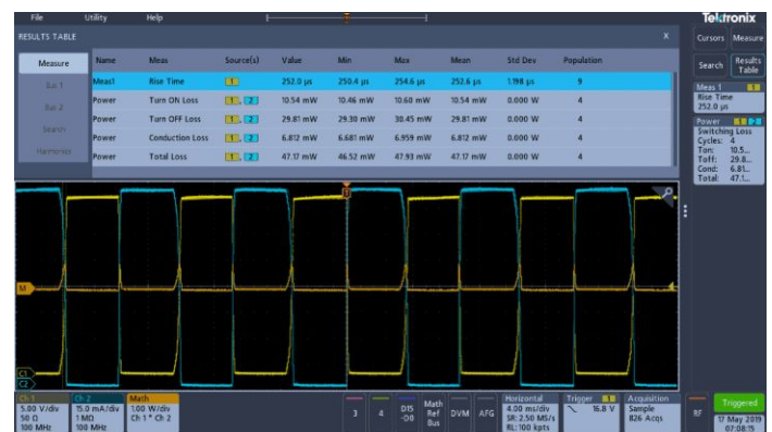
Switching loss measurements
