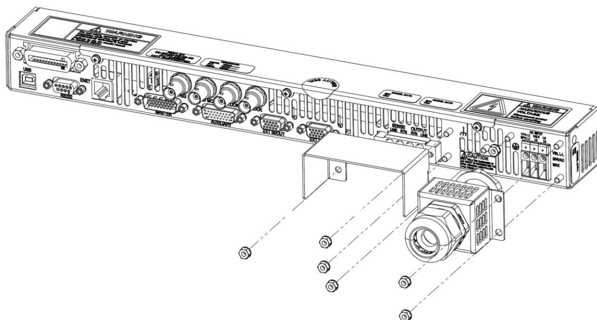
Figure 3-2. Rear Panel Protective Cover Installation
