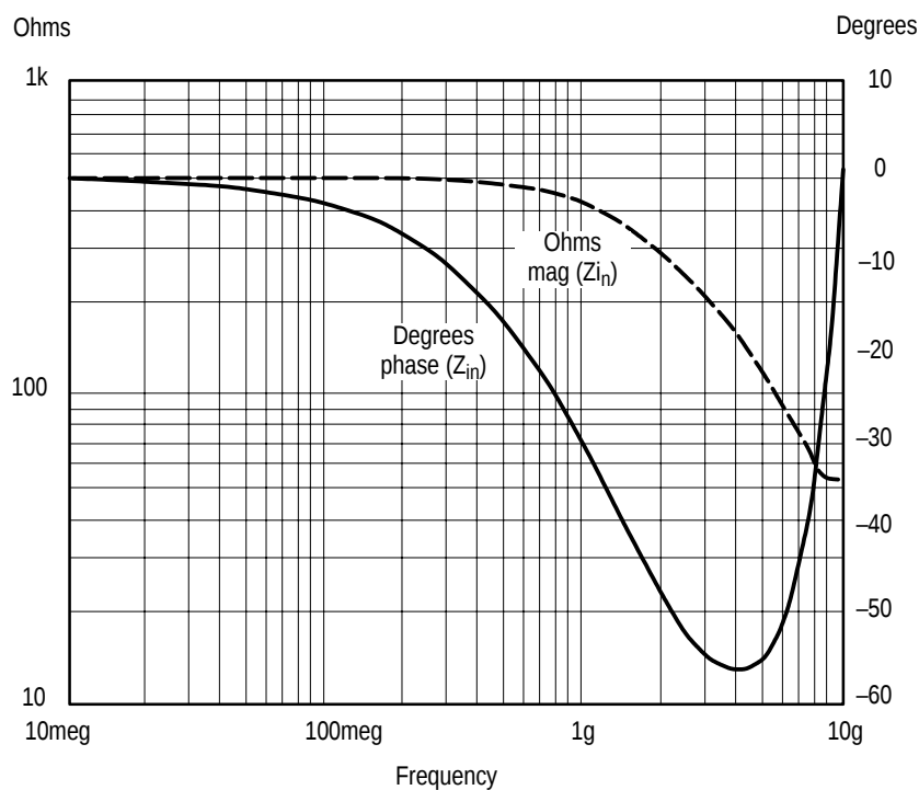
Figure 3: Input impedance
