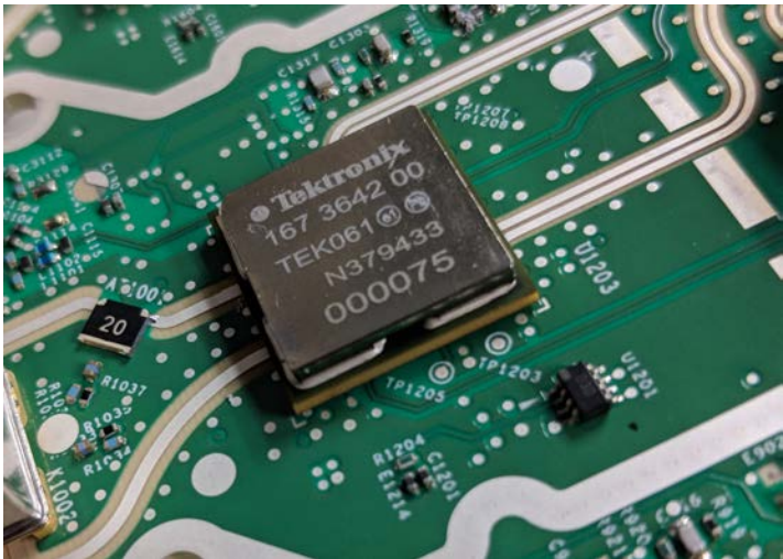
A new TEK061 front end amplifier sets a new standard for low-noise acquisition providing the best signal fidelity to capture small signals with high resolution.
