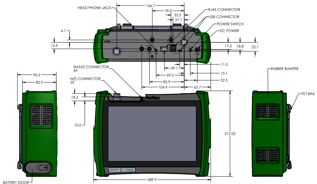
MS2070A
