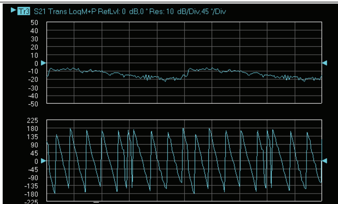
Figure 4-18. Trace Graph - Rectilinear Paired - Trace Log Magnitude and Phase Trace Display Graph
