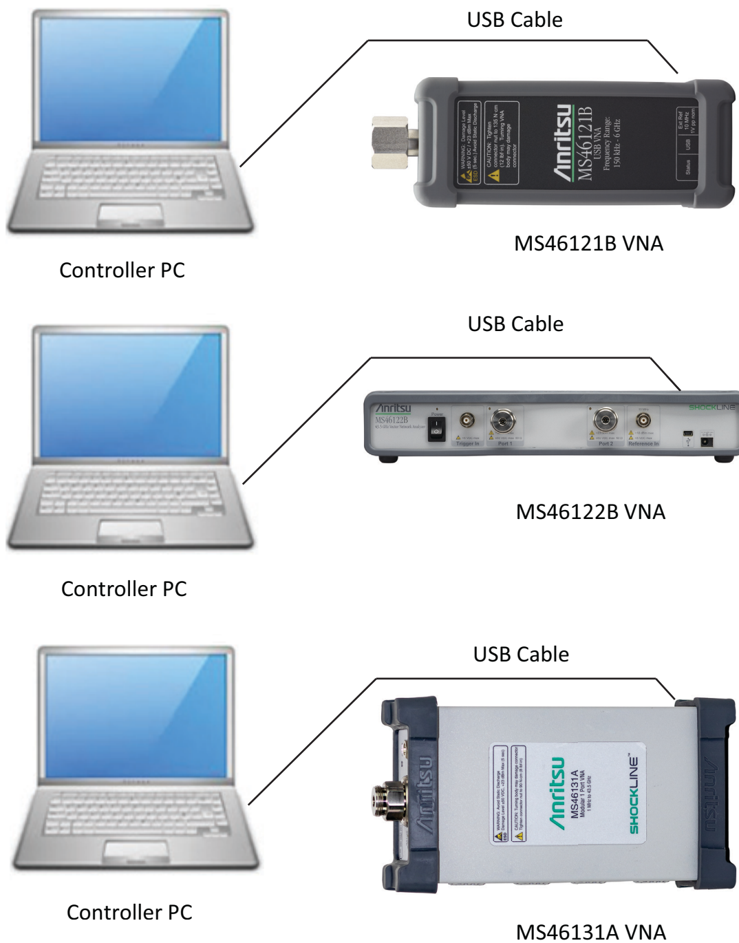
Figure 1-13. Connecting the ShockLine VNA (MS46121B, MS46122B, MS46131A)
