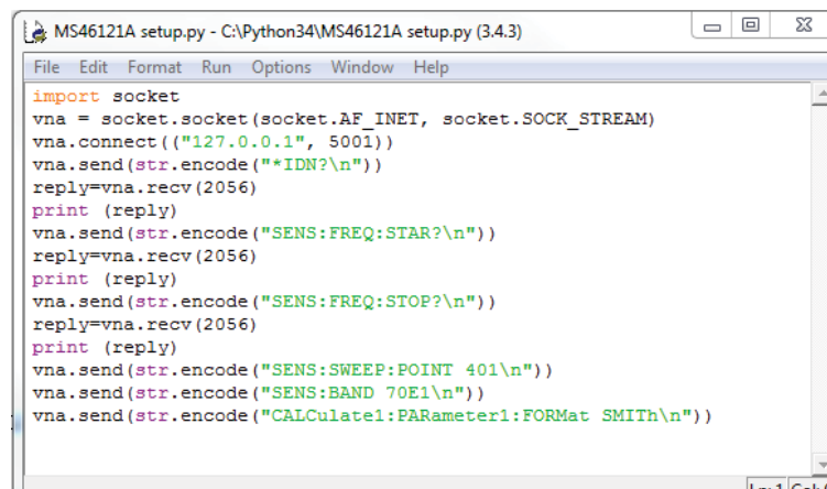
Figure 1-11. Execution of the MS46122A/B Python Script
