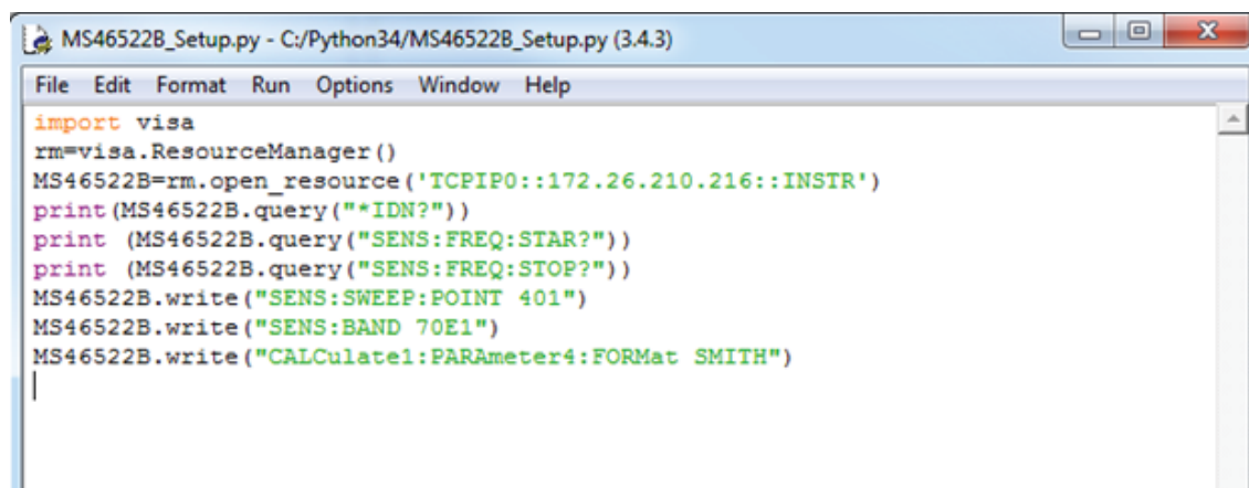
Figure 1-17. Python Script with SCPI Commands
