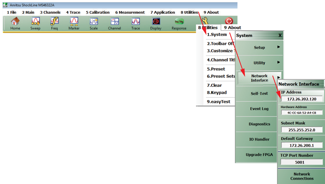
Figure 1-15. IP Address Menu Navigation Path
