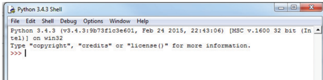
Figure 1-12. Python Shell
