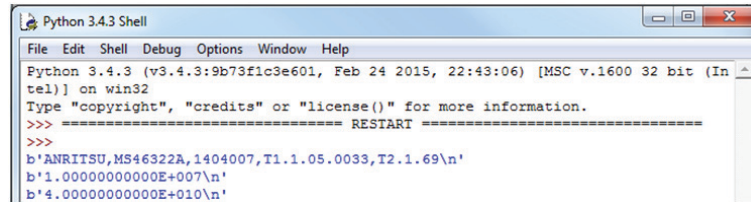
Figure 1-10. Python Script with SCPI Commands for the MS46122A/B
