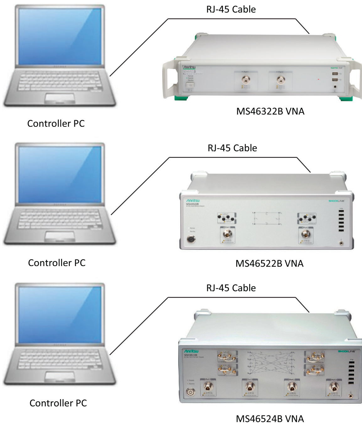
Figure 1-14. Connecting the ShockLine VNA (MS46322B, MS46522B, MS46524B)
