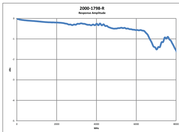
Passband
