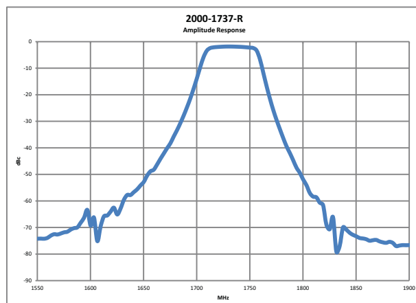
Passband
