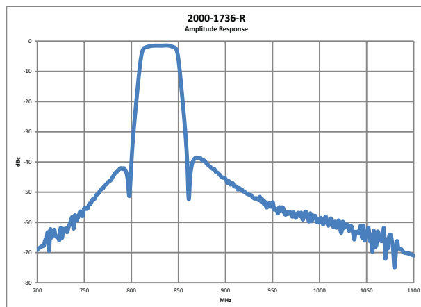
Passband
