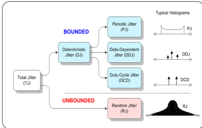
Jitter tree
