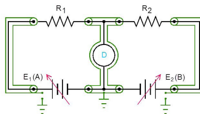
Figure 1. Bridge Block Diagram
