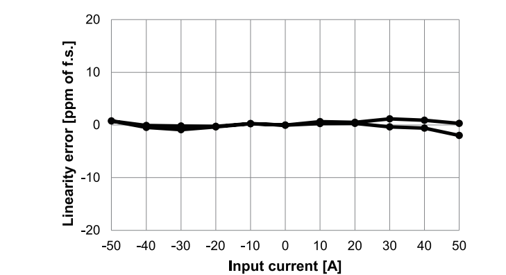
Linearity error (Typical)
