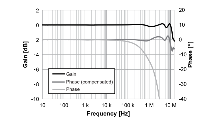
CMRR (Typical)
