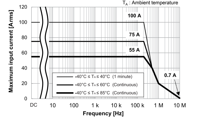
Figure 1. Frequency Derating Curve
