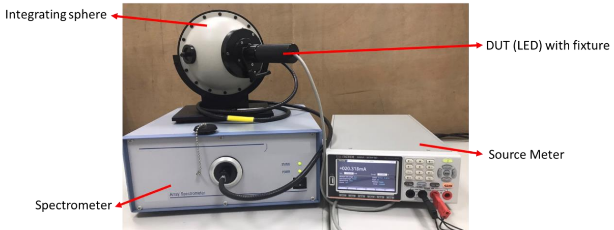
LED Test System Using GW Instek GSM-20H10 Source Meter
