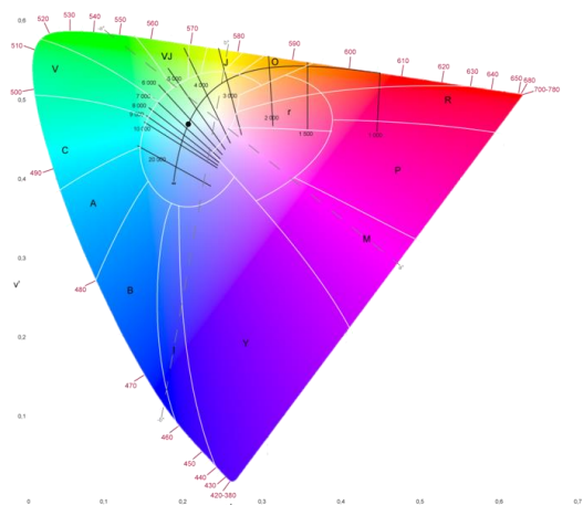
CIE1976 Color Space
