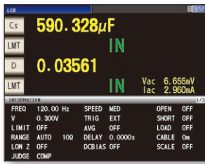
LCR mode Cs and D display screen (120 Hz measurement)
