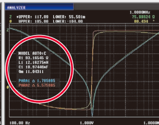
Analysis results simulation screen
