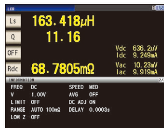
L/Q/Rdc continuous measurement screen L/Q (1 kHz, 1 mA constant current measurement) and Rdc (DC measurement) display screen
