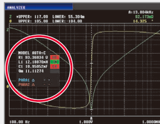
Acceptance/rejection decision screen for equivalent circuit elements
