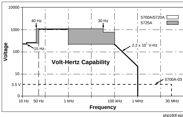
Figure 1-1. Volt-Hertz Capability
