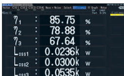
PW3337
