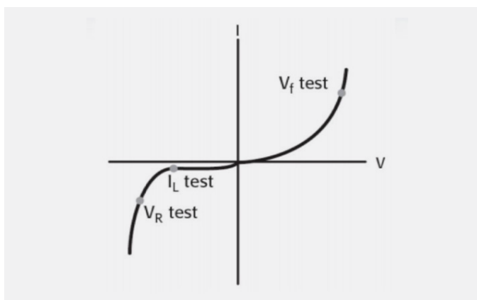
FIGURE 6. Typical HBLED DC I-V curve and test points for manufacturing tests (not to scale).
