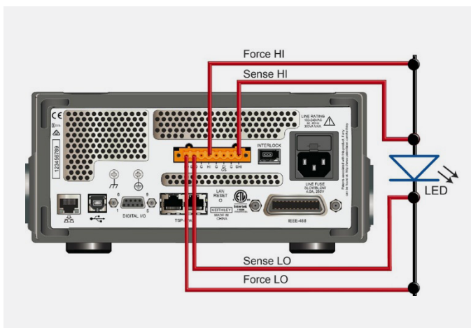
FIGURE 5. 2461 4-wire rear-panel connections to an LED.
