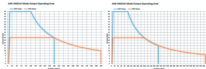
AC Output for ASR-3400/3400HF
