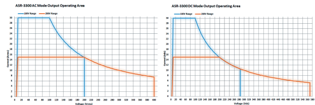
AC Output for ASR-3300
