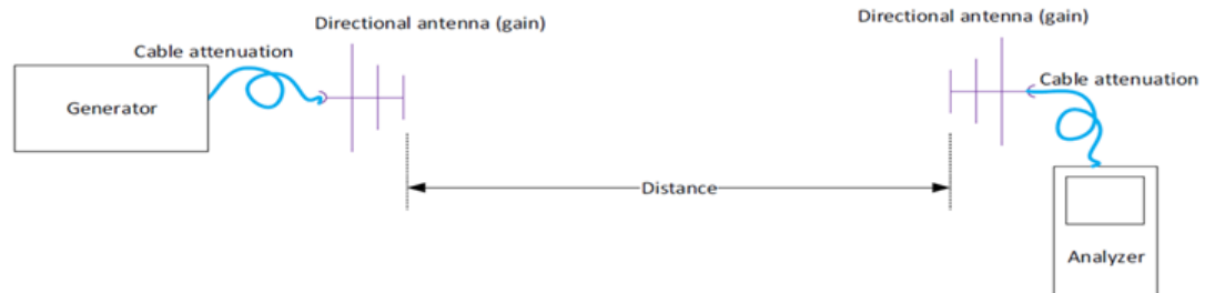
Figure 6-11: Test setup for EIRP measurement
