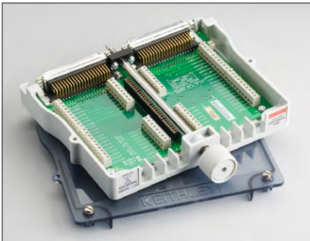
3732-ST-R: Screw Terminal Block. Enables screw terminal access and additional matrix sizes including: dual 8x28 (1W), single 8x28 (2W), and single 16x28 (1W).
