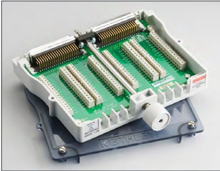
3732-ST-C: Screw Terminal Block. Enables screw terminal access and additional matrix sizes including: quad 4x28 (1W), dual 4x28 (2W), single 4x56 (2W), dual 4x56 (1W), and single 4x112 (1W).
