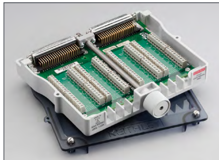
3723-ST: Screw Terminal Block. Accessory for 3723 for two-pole applications.
