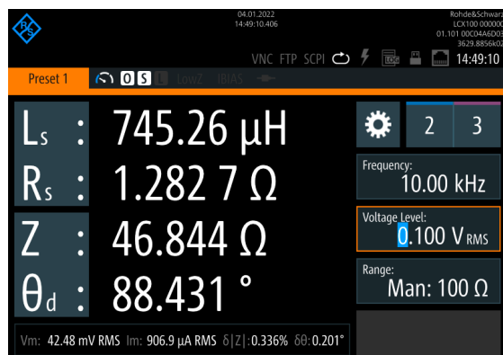
Primary inductance measurement at 10 kHz and 100 mV (RMS)
