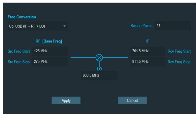
Mixer configuration setup.
